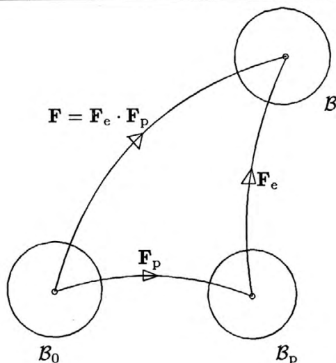
Figure 2: The intermediate configuration \mathcal{B}_p is obtained from the deformed configuration \mathcal{B} by destressing to zero stress. The elastoplastic deformation gradient is decomposed into elastic and plastic parts, such that \mathbf{F} = \mathbf{F}_e \cdot \mathbf{F}_p .
